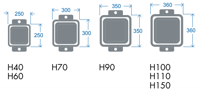
CROSS SECTION DETAILS HEAVY OF FRAME
